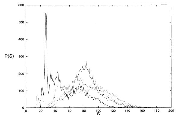
FIG. 6. Plot of four distributions P(S) of the number S of sites visited by random walks starting at four different points of the percolating cluster at the critical threshold. Each distribution is made from 10 000 realizations of walks of n = 1000 steps which start at a fixed origin. The lattice size here is 250 \times 250 .
