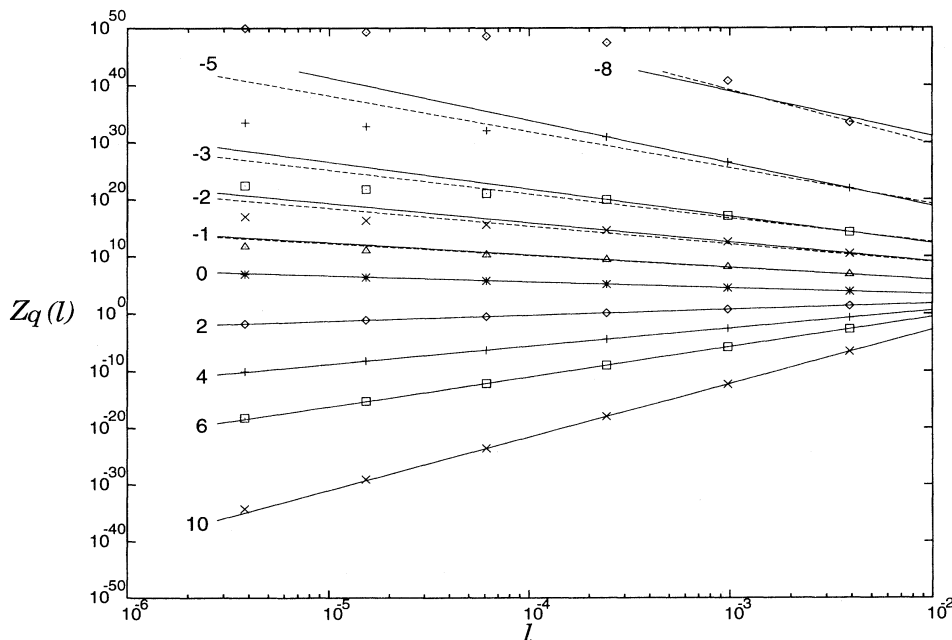
FIG. 4. Plot of Z_q(l) versus l in a log-log representation, for different q values ( q values are shown at the left of the curves). The symbols are the calculated Z values, while the continuous lines are the fits to the data. The dotted lines are the homogeneous slopes \tau_h(q) = q - 1 . Note the crossover in the slopes of the negative moments, which occurs at about \nu = 12 .
