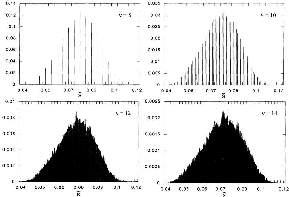
FIG. 3. Histogram of the probabilities of occurrences of \bar{s} values for four box subdivisions, as shown in the figures. The data were obtained from the lattice of size 750 \times 750 .
