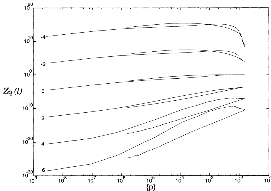
FIG. 9. Plot of the partition function Z_q(l) as a function of the first moment \{p\} \equiv m_1 , for different values of q ( q values are shown at the left of the curves).
