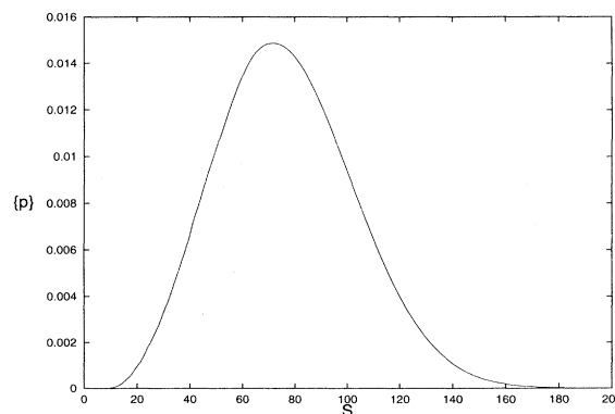
FIG. 8. Plot of the distribution of the first moment of p , i.e., the average value \{p\} \equiv m_1 , with regard to the number of sites visited, for a walk of n = 1000 steps, for 12 different realizations of the percolation cluster.
