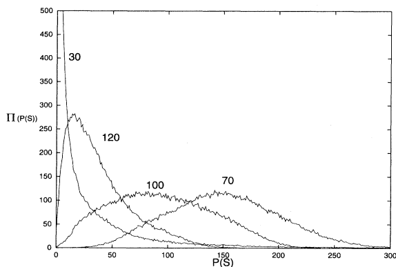
FIG. 7. Plot of the distributions \Pi of the probabilities P(S_n) when all the origins of 12 different realizations of the percolation cluster are taken, resulting to a total of almost 180 000 origins. Four values of S_n are considered, as marked. The x axis in this figure corresponds to the y axis of Fig. 6. The y axis in this figure now shows the distribution of the P values for about 180 000 different origins for the four specific S_n values. For each origin P(S_n) was determined with n = 1000 steps and 10 000 realizations of the walks, as the data in Fig. 6.
