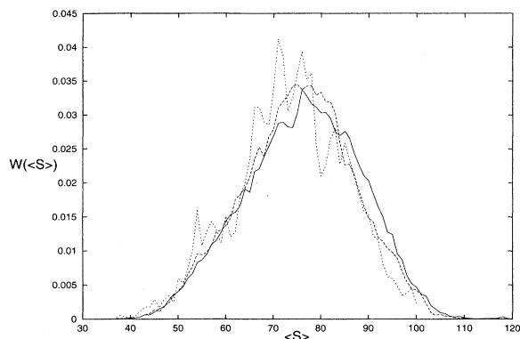
FIG. 1. Distribution W of \langle S_n \rangle , the mean number of distinct sites visited by random walks in the infinite cluster of a percolating lattice. The solid line represents the distribution for a cluster of size 750 \times 750 , where N_r = 180\,605 , the dotted line represents the distribution for a cluster of size 250 \times 250 with N_r = 14\,550 , while the dashed line represents the average of 12 different clusters of size 250 \times 250 .
